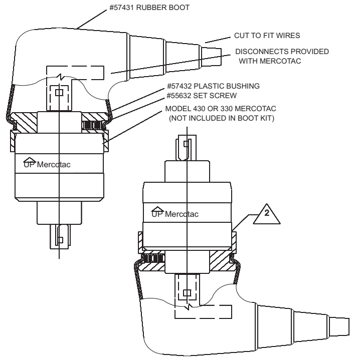
#57430 BOOT KIT
