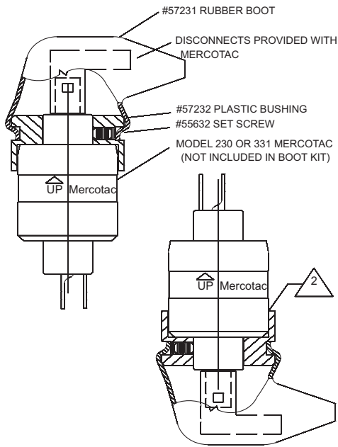
#57230 BOOT KIT
